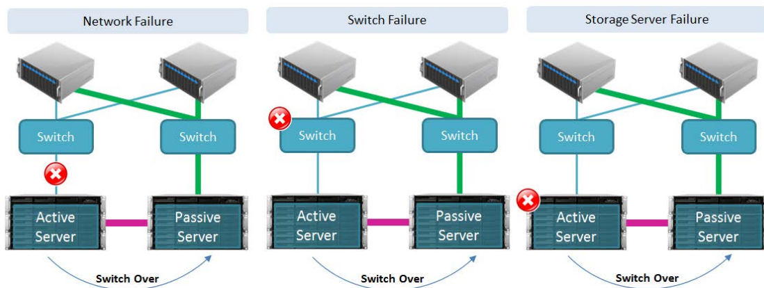
Figure 3: High-availability cluster network configuration on models with two LAN ports
