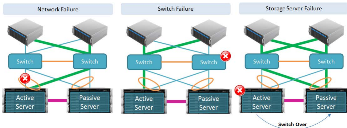
Figure 5: High-availability cluster network configuration on models with four or more LAN ports (NAS)
